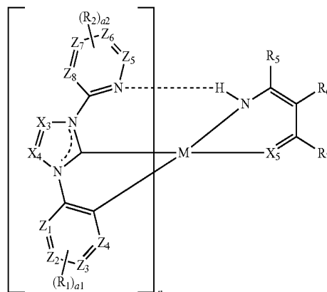
Formula 10
