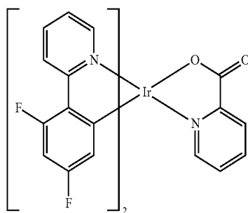
Flrpic
