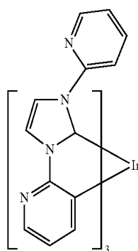
Compound B
