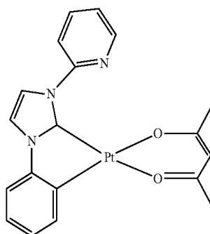
Compound C
