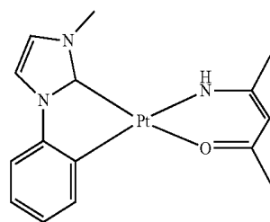
Compound A
